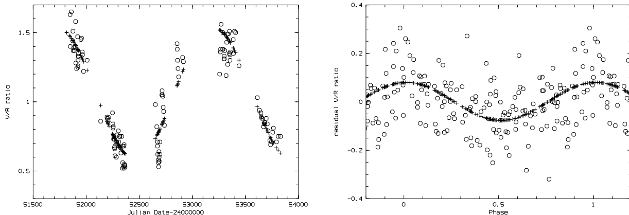
Figure 4. H \alpha V/R -ratio. Left: The measured values vs. Julian date (open symbols) and the sine wave with \mathcal{P} = 1471 d (plus signs). Right: The residuals of the left panel, folded with \mathcal{P} = 69.3 d and the respective sine fit. Shown are 1.4 cycles for clarification, i.e. 40 % of the points are redundant.
