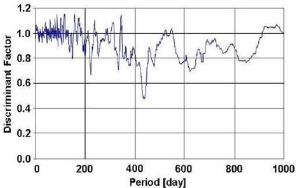
Figure 6. PDM analysis of the time series in Fig. 4
