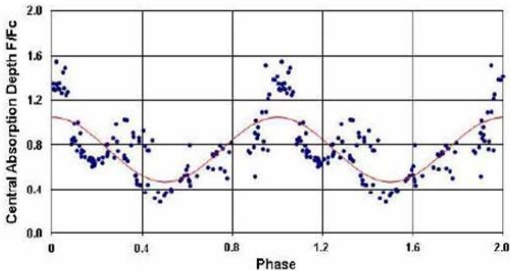
Figure 5. Phase plot of the PDM analysis in Fig. 6; Period = 442 d ( \pm 5 ), Epoch = JD 2455571 ( \pm 16 )
